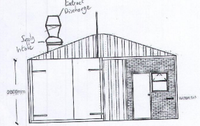
EAST ELEVATION
